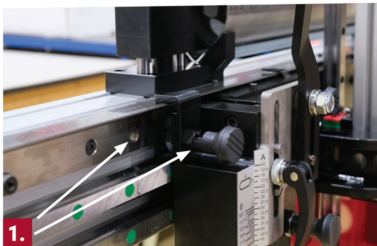
1. Easy and exact pin-to-hole positioning, with index plate at two customised intervals.
